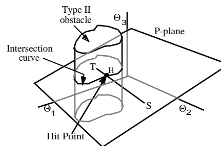
Figure 7. Type II obstacle forms a generalized cylinder in C-space.
