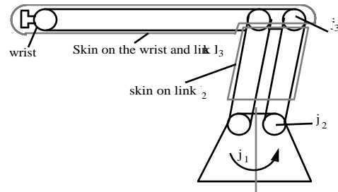
Figure 1. Sketch of robot arm and sensor skin.
