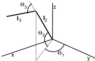
Figure 4. Sketch of robot arm configuration
